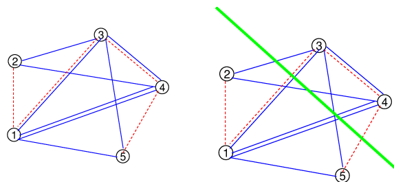
Figure 2: Left: The graph induced by the quartets ((1, 2), (3, 4)) and ((1, 3), (4, 5)) from Figure 1. Right: A cut separating \{1, 2, 5\} from \{3, 4\} , therefore satisfies quartet ((1, 2), (3, 4)) but violates ((1, 3), (4, 5)) and hence contains 6 good and 2 bad edges.
