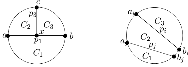
Figure 1: One of the cycles C_1, C_2 and C_3 is even.
