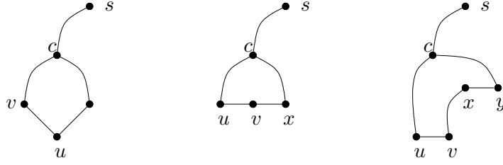
Figure 3: The even cycles detected by rules 3,5 and 6
