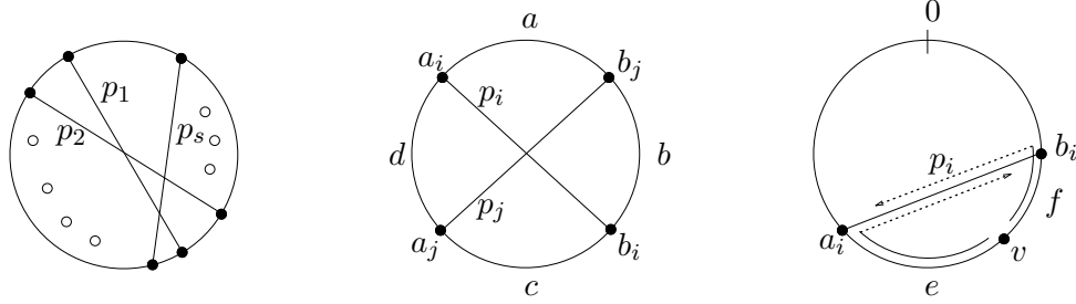
Figure 2: The shortcuts of P .
