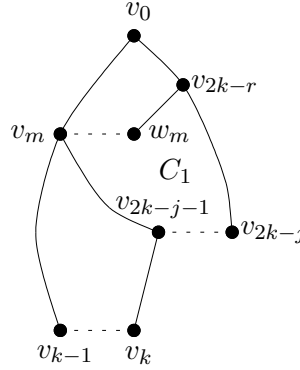
Figure 4: If \rho(v_k) = \rho(v_{k-1}) = v_m then |C_1| = 2(j - r + 1) < 2k
